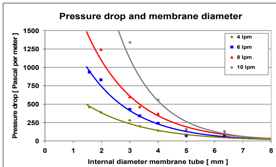
Figure 2: The pressure drop versus internal diameters of a single hollow fiber PDMS membrane at gas flow rates of 4, 6, 8 and 10 liters per minute.
